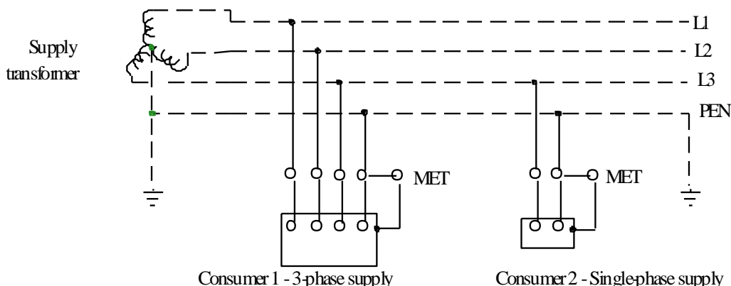
TN-C-S system (also known as PME supply)
