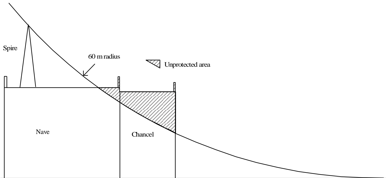
Figure 1 – Unprotected area with spire-only protection
