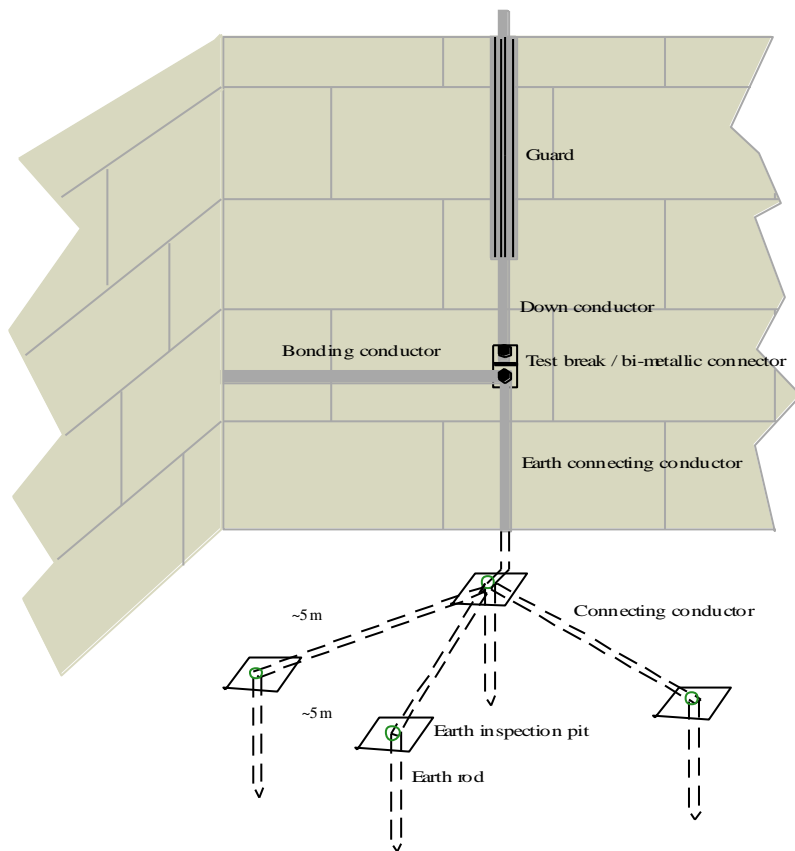
Figure 5 – A possible layout of conductors earthing conductors
