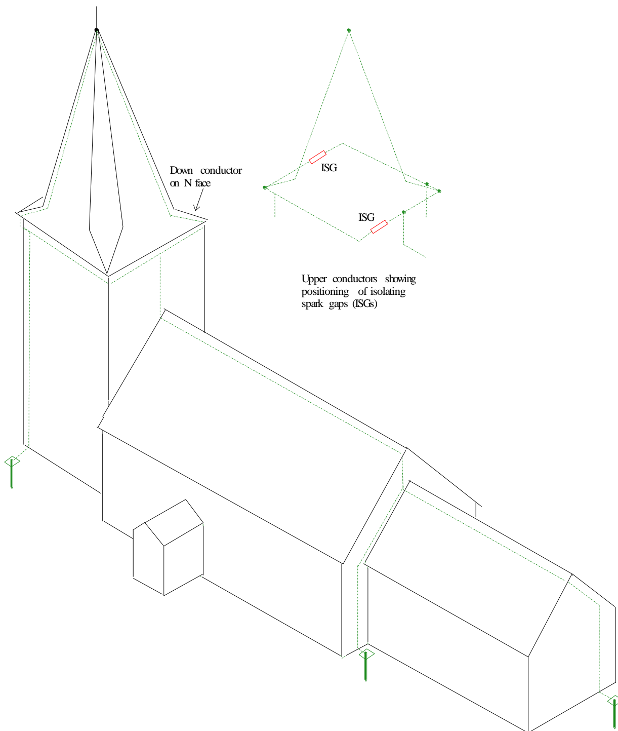
Figure 3 – Layout of a typical smaller parish church installation
