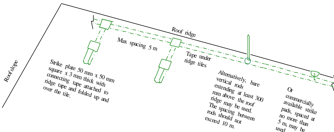
Figure 2 – Air terminations for ridge conductor placed under the ridge tiles
